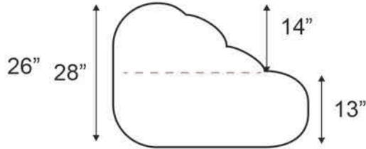
Side View of Cuddle Seat
